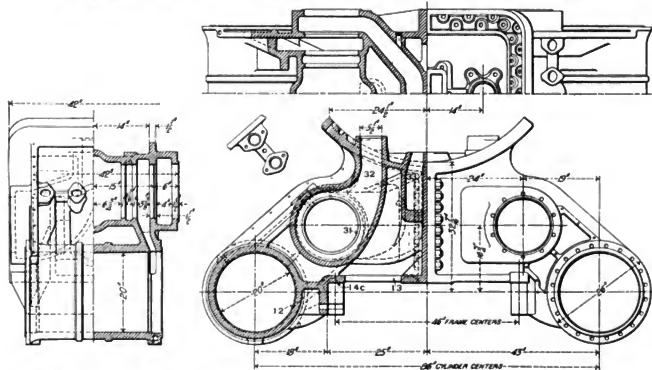
Figs. 804-807. Cylinders for Simple Locomotive with Piston Valves, Diameter 20 in. American Locomotive Co.
